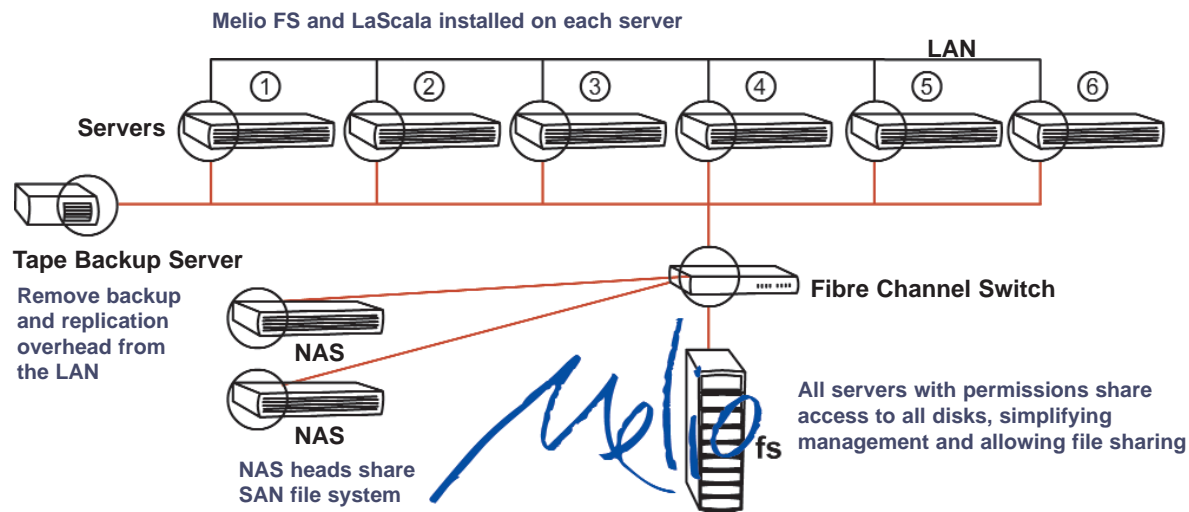
Diagram of Melio FS in a Workgroup Environment
